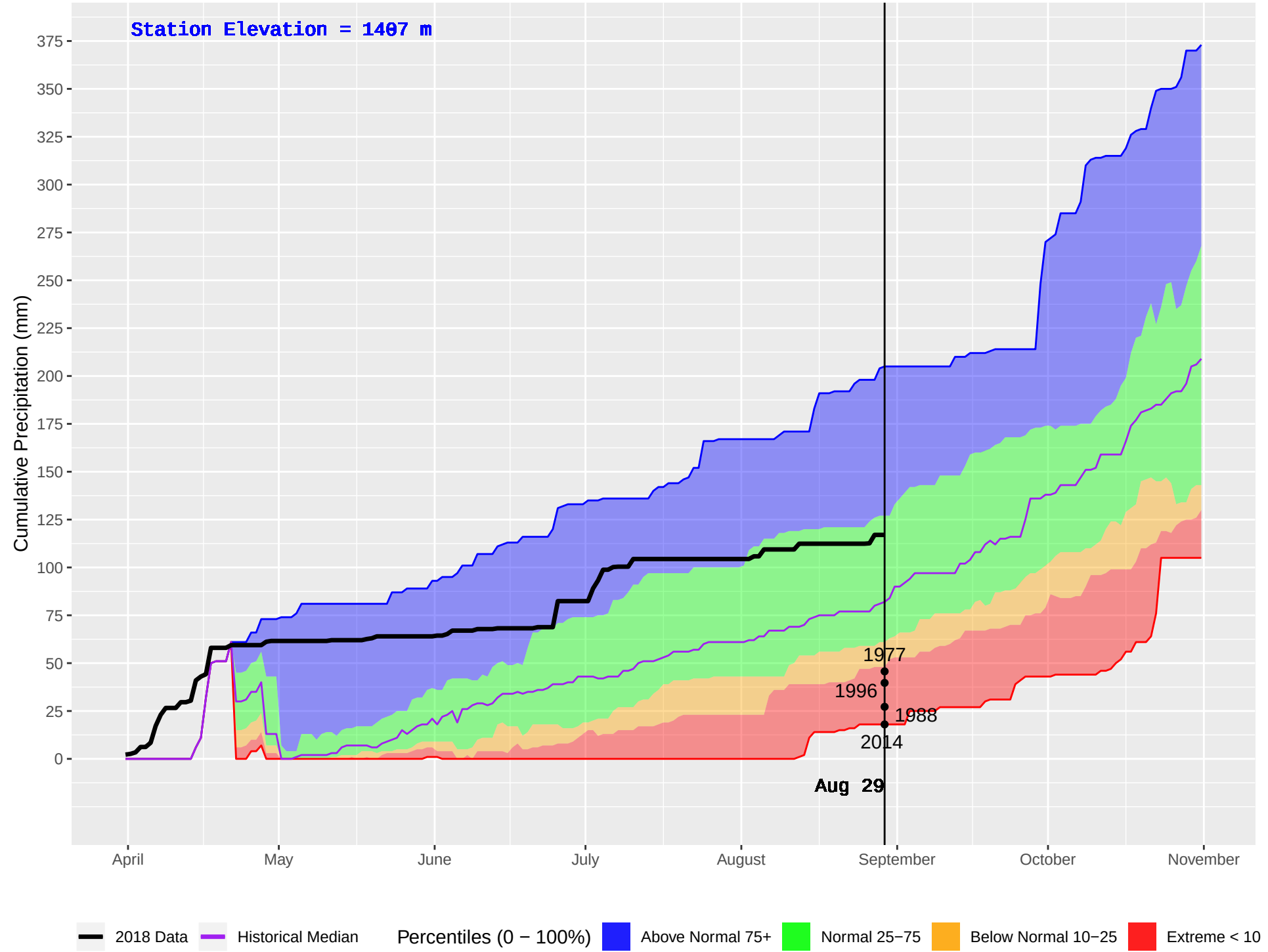
THYNNE (279) : Historical (1977–2016) and Current (2018) Daily Cumulative Precipitation
