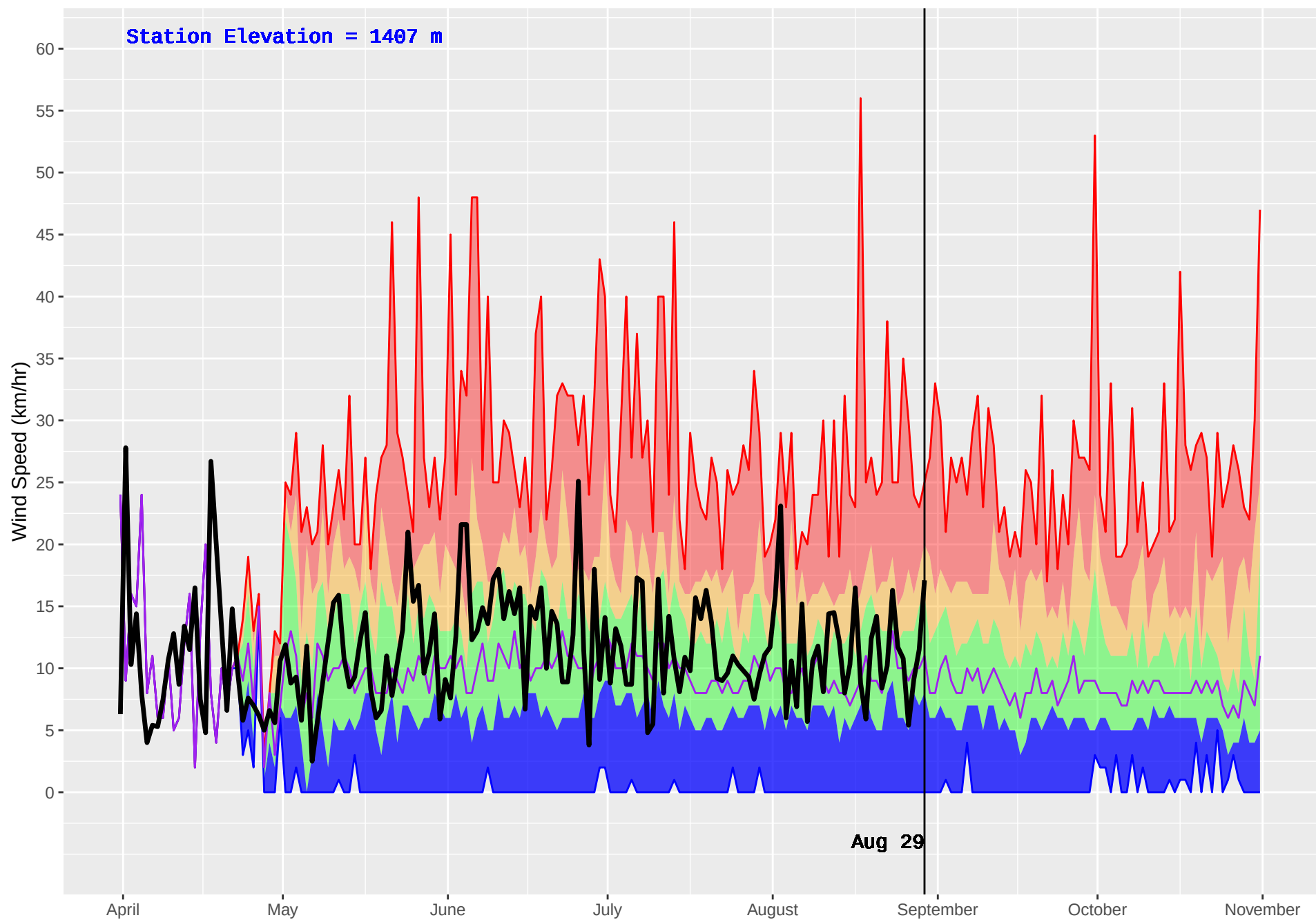
THYNNE (279) : Historical (1977–2016) and Current (2018) Daily Wind Speed
