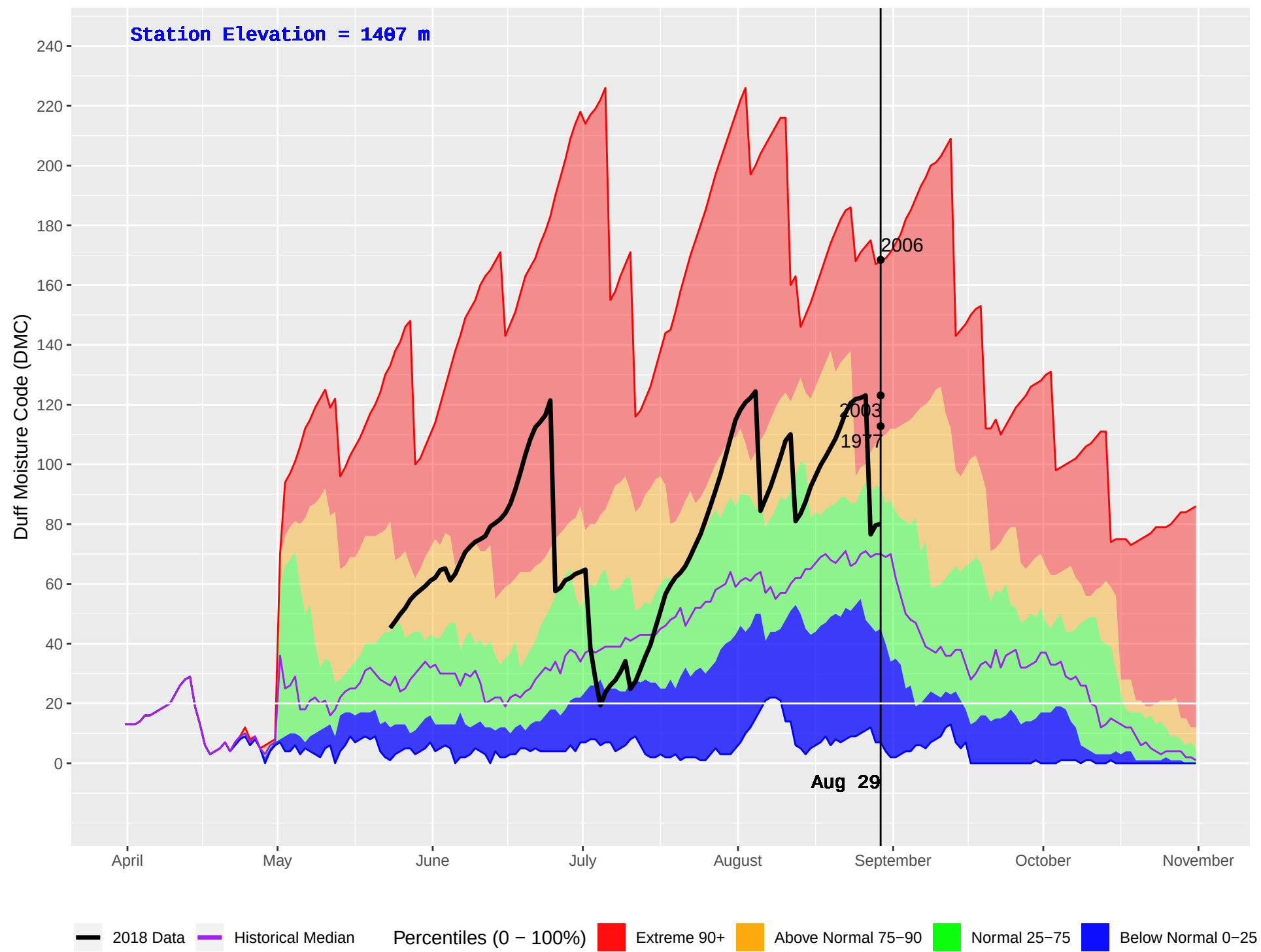
THYNNE (279) : Historical (1977–2016) and Current (2018) Daily Duff Moisture Code (DMC)
