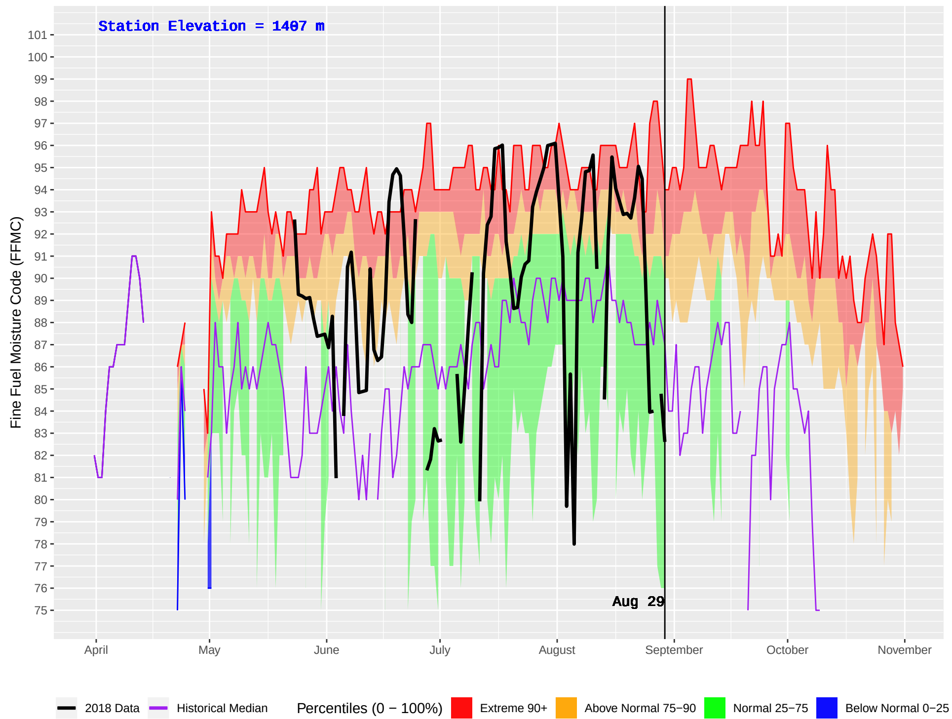
THYNNE (279) : Historical (1977–2016) and Current (2018) Daily Fine Fuel Moisture Code (FFMC)
