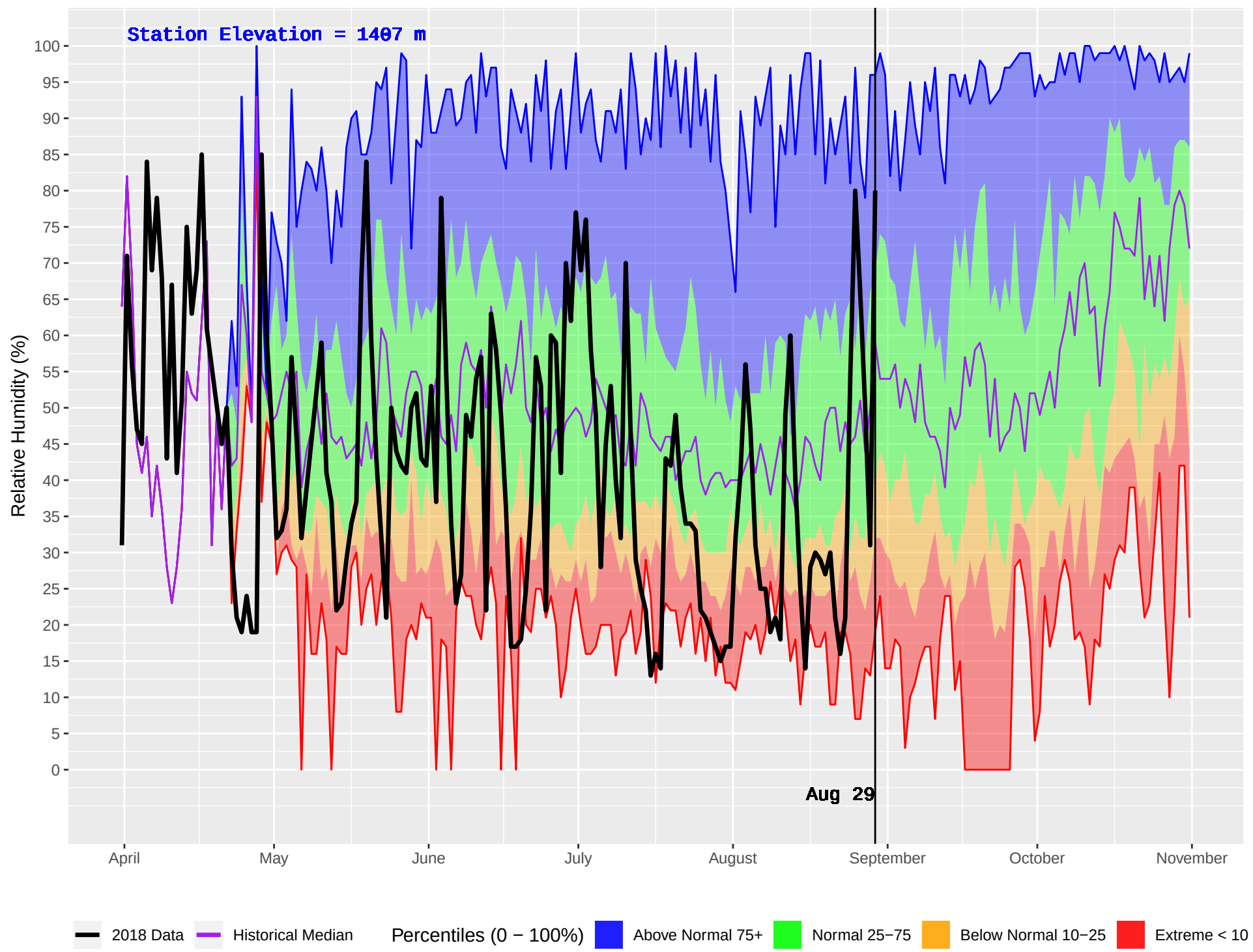
THYNNE (279) : Historical (1977–2016) and Current (2018) Daily Relative Humidity
