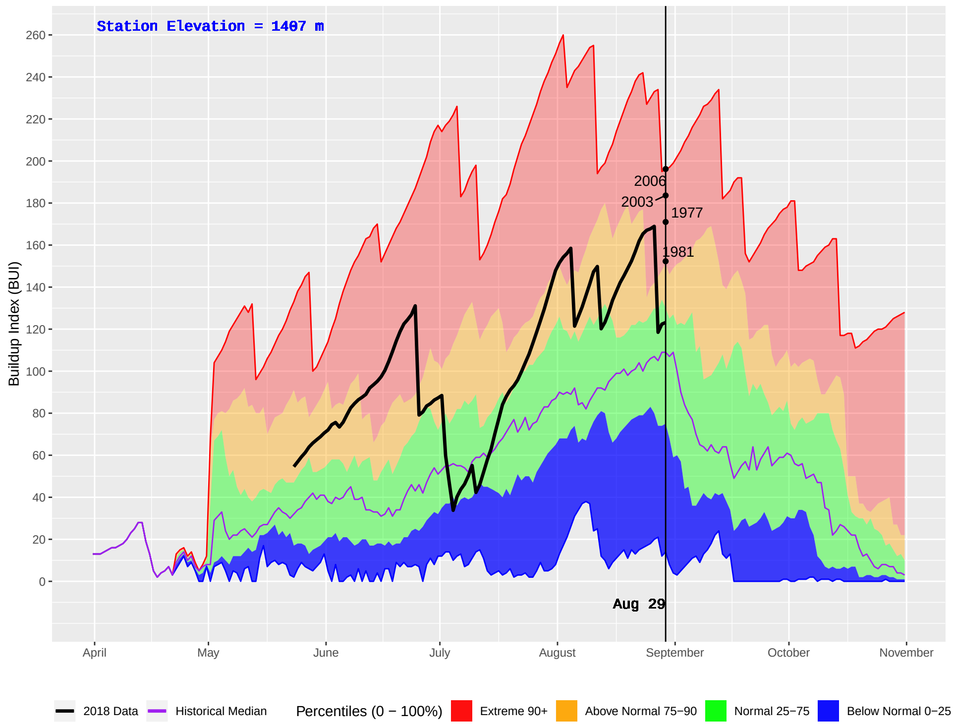
THYNNE (279) : Historical (1977–2016) and Current (2018) Daily Buildup Index (BUI)
