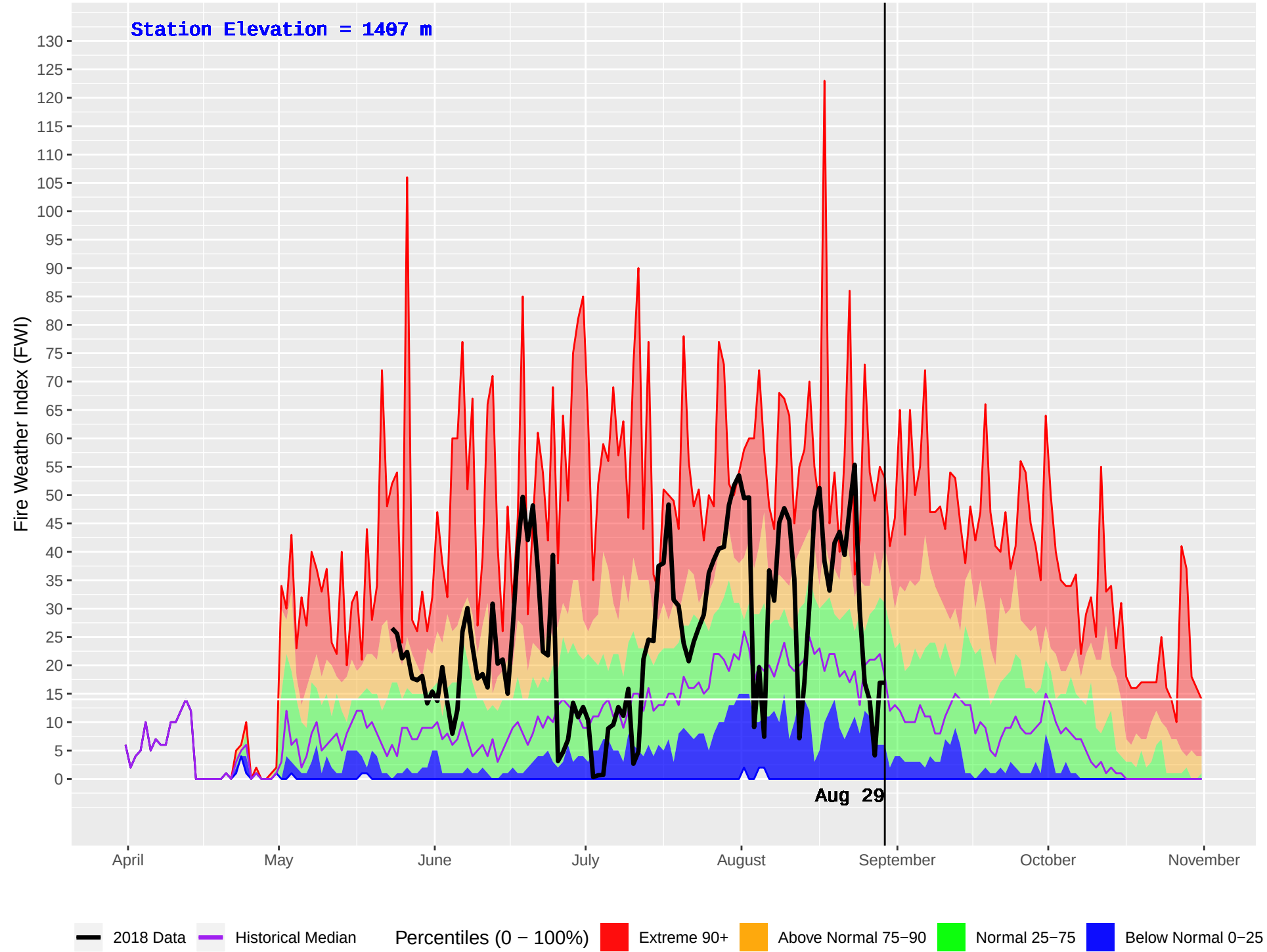
THYNNE (279) : Historical (1977–2016) and Current (2018) Daily Fire Weather Index (FWI)
